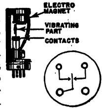
Vibrator construction and symbol.
